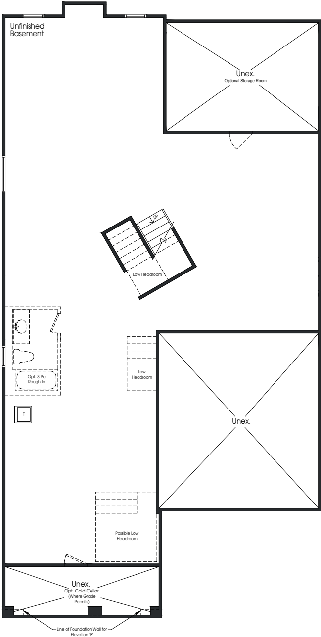
QUEENSPORT II BUNGALOW WITH OPTIONAL LOFT BASEMENT PLAN 'A' & 'B'
