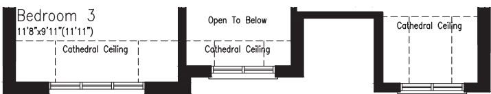
PARTIAL SECOND FLOOR PLAN 'C'
