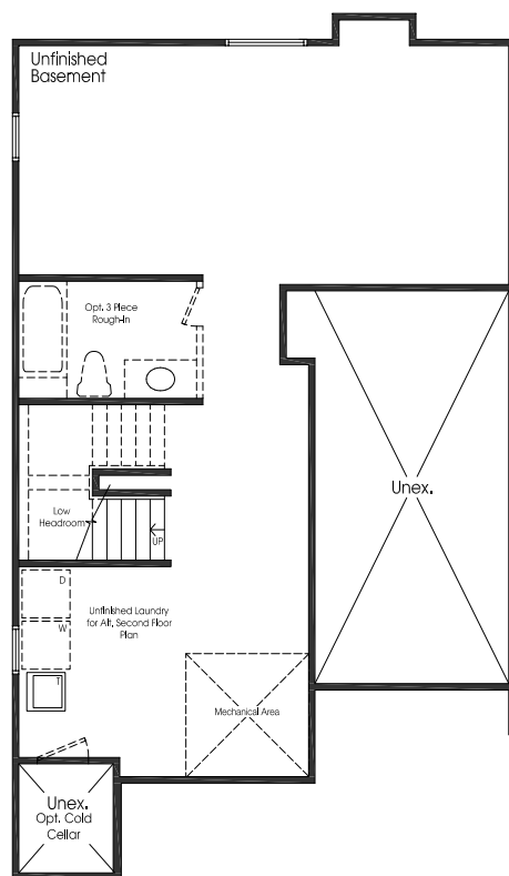
BASEMENT FLOOR PLAN 'A'
