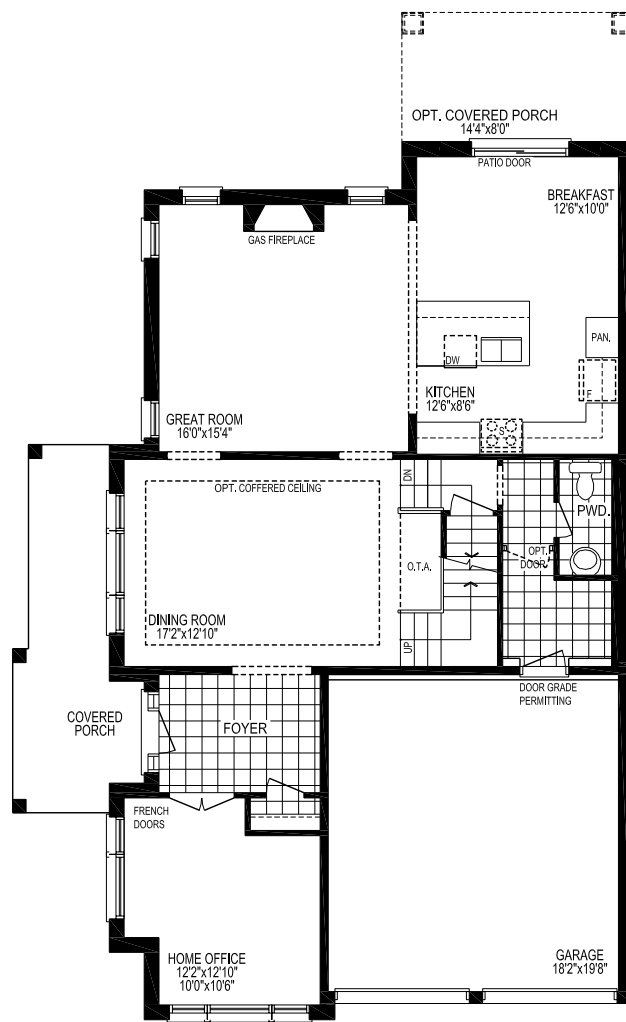
GROUND FLOOR PLAN EL. 'B' ('C' SIMILAR)
