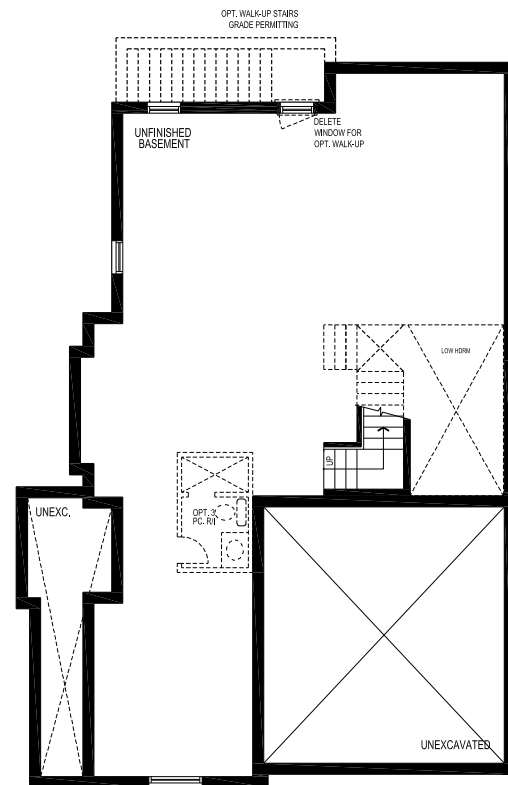
BASEMENT PLAN EL. 'A' & 'C' ('B' SIMILAR)
