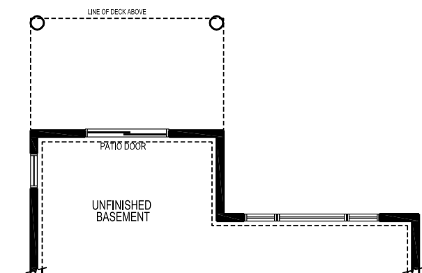
PART. BASEMENT PLAN EL. 'A', 'B', 'C', & 'D' - WALK-OUT CONDITION
