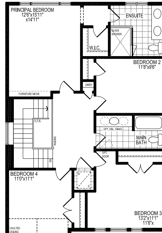
ALT. SECOND FLOOR PLAN, EL. 'A' W/ 4 BEDROOM ('D' SIMILAR)
