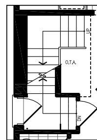
PART. GROUND FLOOR PLAN FOR SIDE DOOR OPTION, EL. 'A', 'B', 'C', & 'D'
