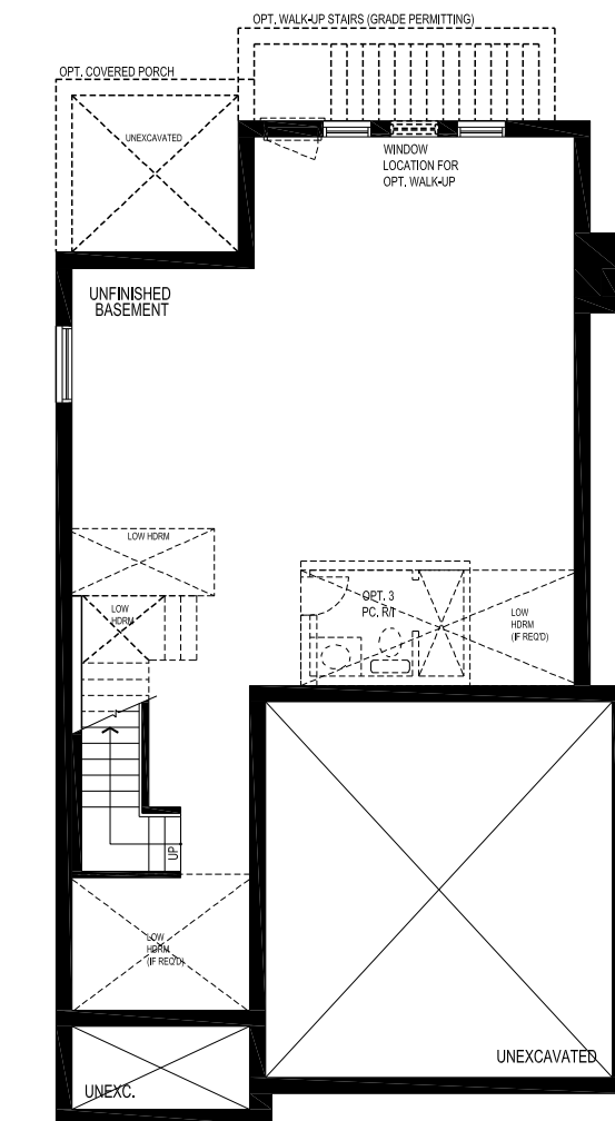
BASEMENT PLAN EL. 'A', 'B' & 'C'
