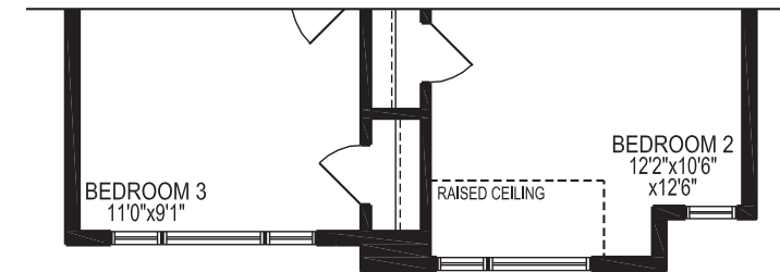
PART. SECOND FLOOR PLAN, EL. 'B'
