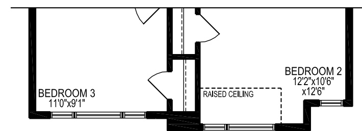
PART. SECOND FLOOR PLAN, EL. 'B'
