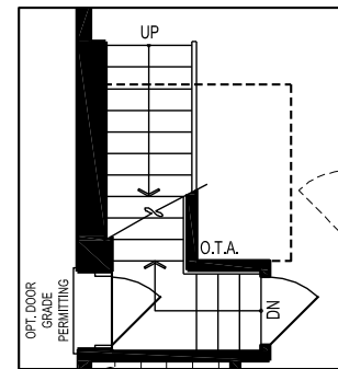
PART. GROUND FLOOR SIDE DOOR
