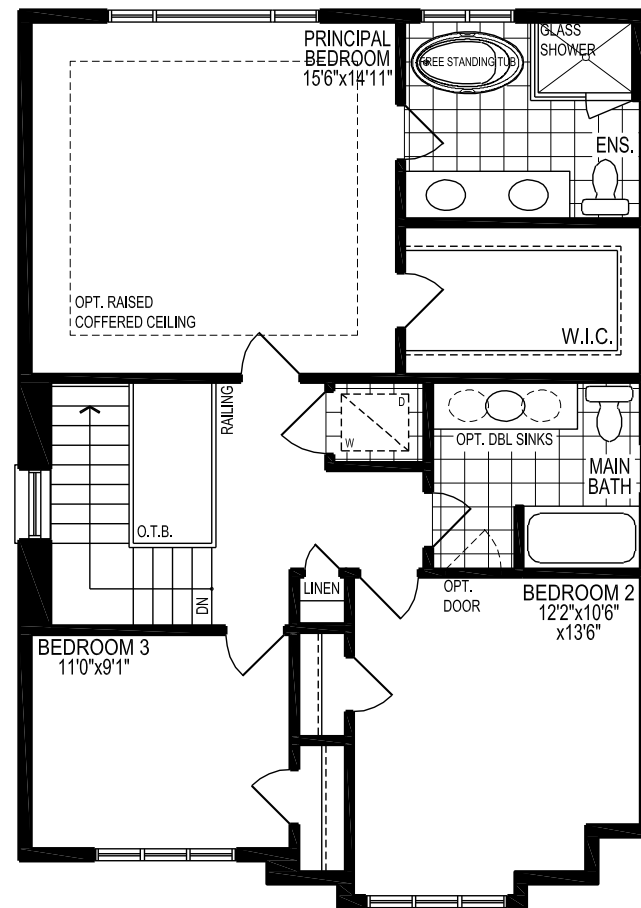
SECOND FLOOR PLAN EL. 'A'
