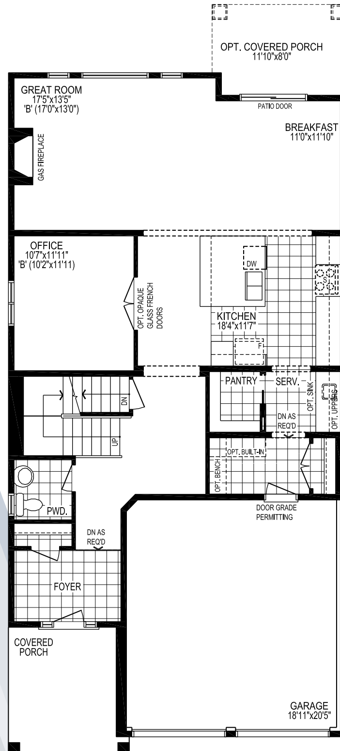
GROUND FLOOR PLAN W/OFFICE, EL. 'A' (B SIMILAR)
