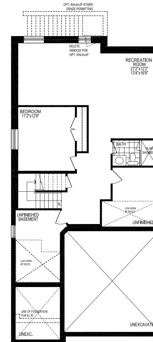
OPTIONAL FINISHED BASEMENT PLAN 'A' & 'B'
