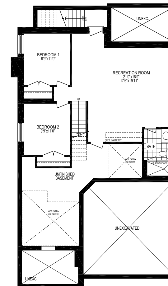
OPT. FINISHED BASEMENT PLAN, EL. 'A' & 'B' WALKUP CONDITION
