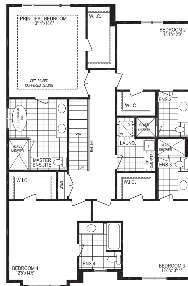
OPT. SECOND FLOOR PLAN EL. 'A'
