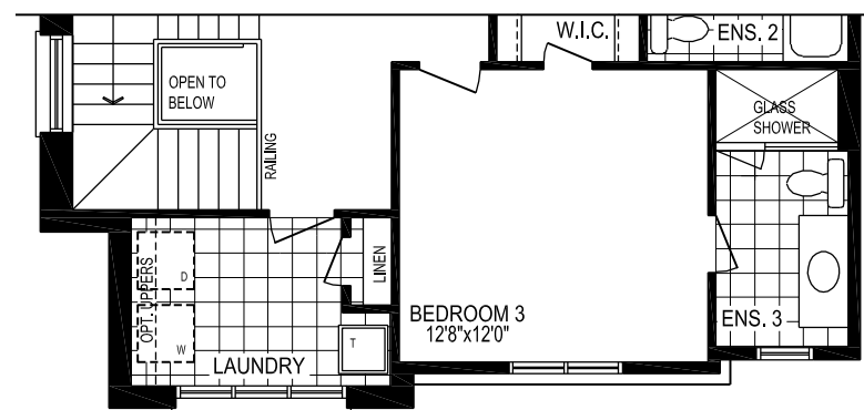
PART. SECOND FLOOR PLAN EL. 'B'
