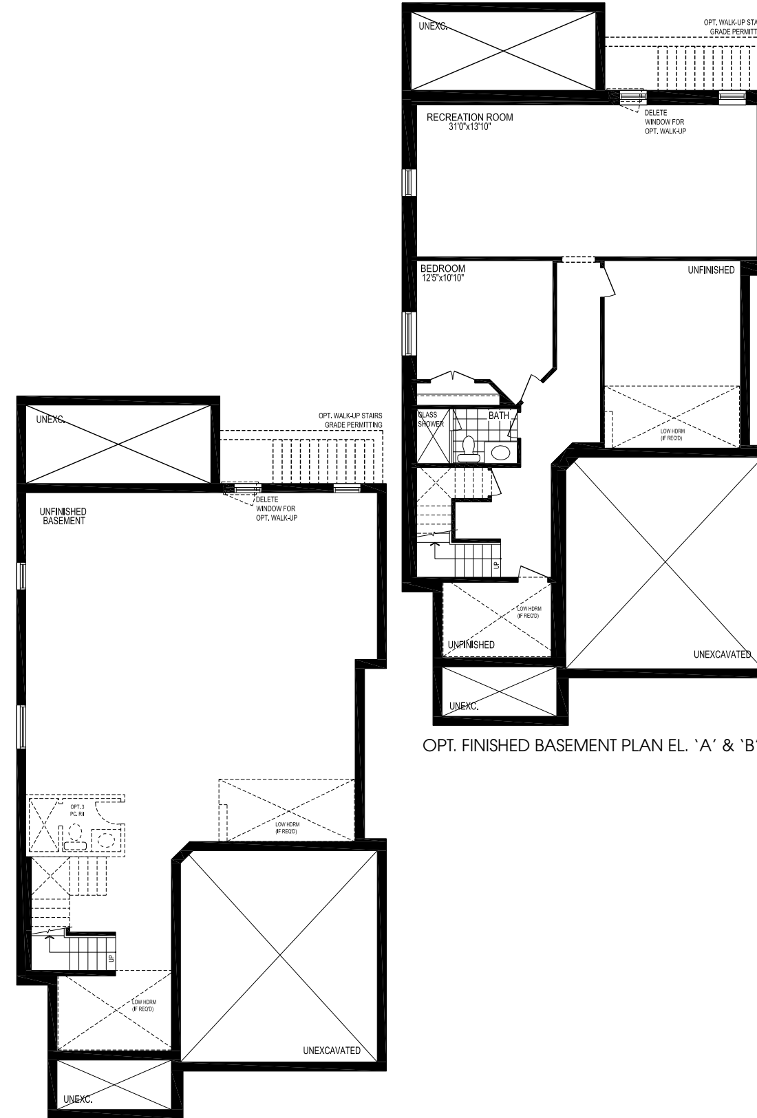
BASEMENT PLAN EL. 'A' & 'B'
