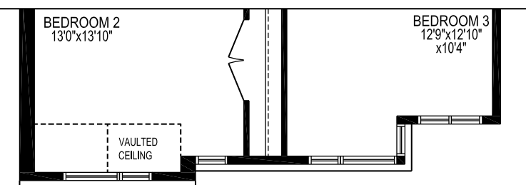
PART. SECOND FLOOR PLAN, EL. 'B' ('C' SIMILAR)
