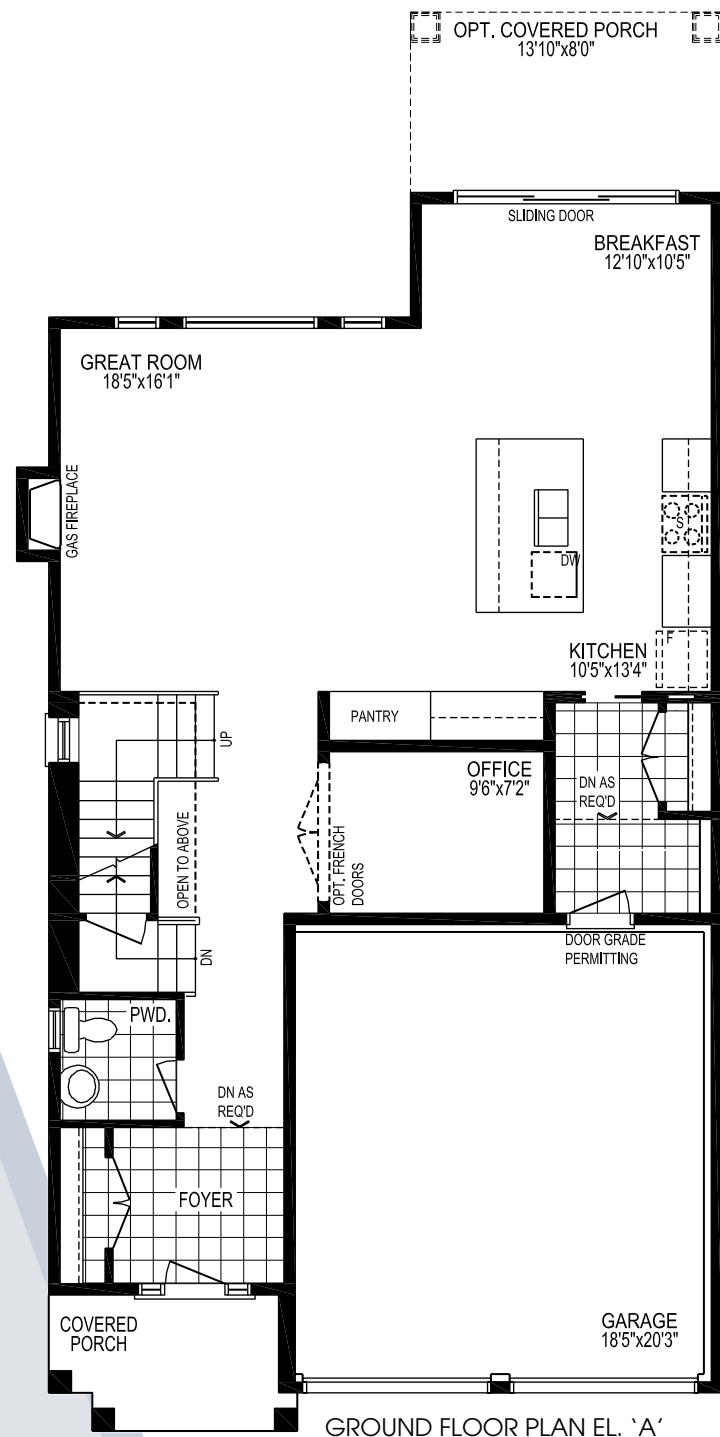
GROUND FLOOR PLAN EL. 'A'
