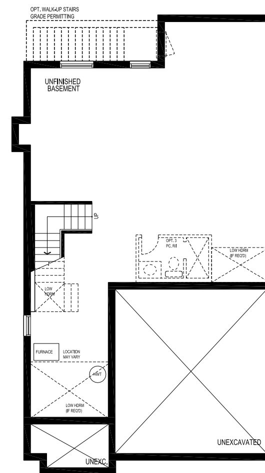
BASEMENT PLAN EL. 'A' & 'C' ('B' SIMILAR)
