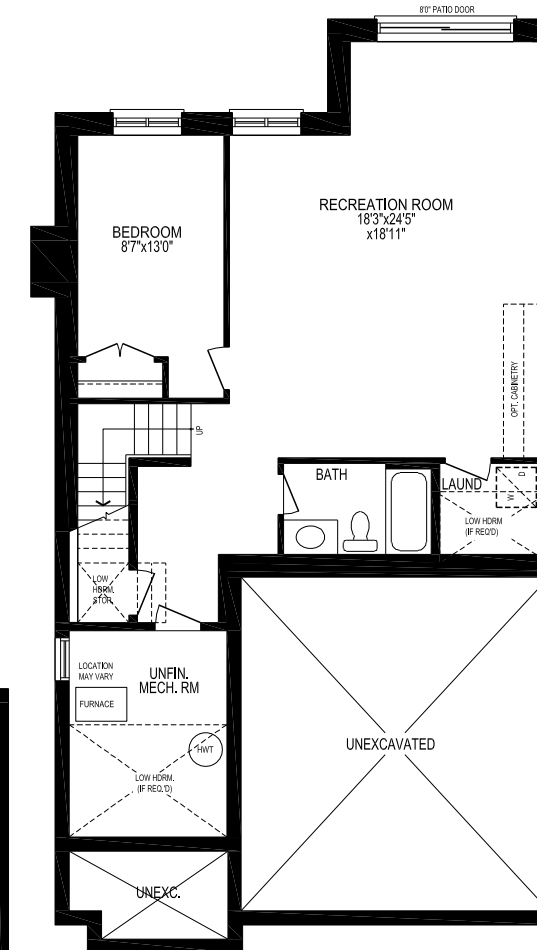
OPT. FINISHED BASEMENT PLAN EL. 'A' & 'C' WALK-OUT CONDITION ('B' SIMILAR)
