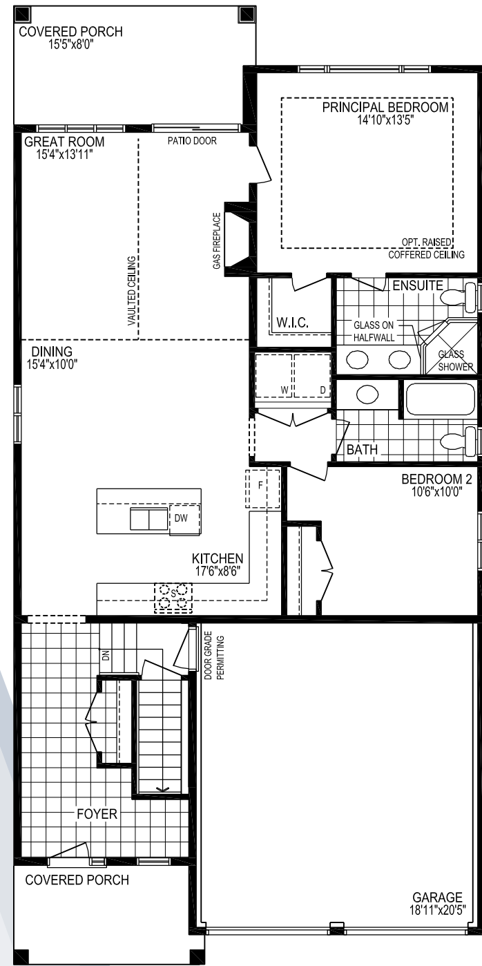
GROUND FLOOR PLAN, EL. 'A' & 'B'
