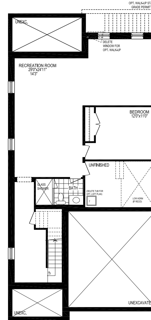
OPT. FINISHED BASEMENT PLAN, EL. 'A' & 'B'
