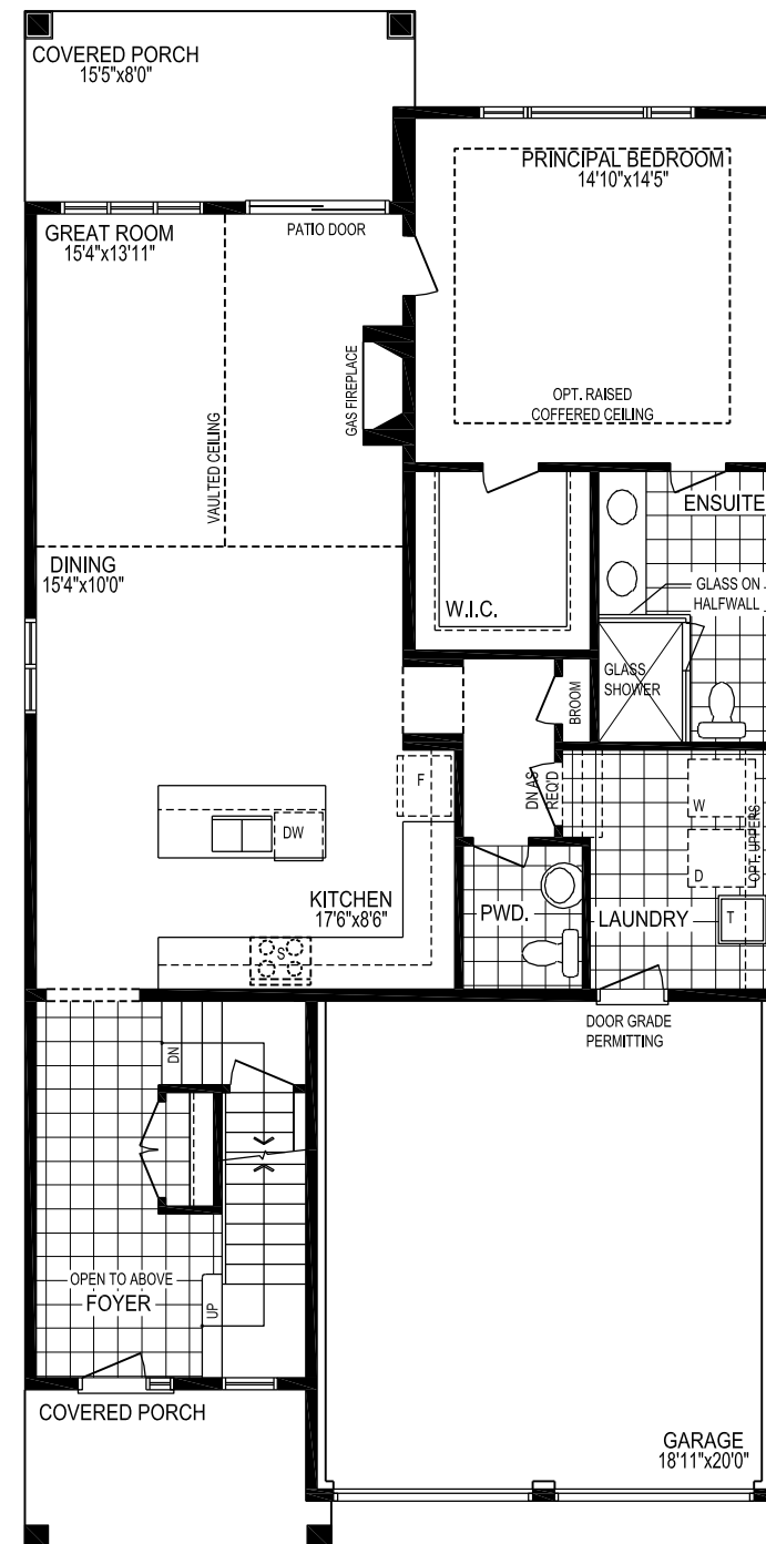
GROUND FLOOR PLAN WITH LOFT, EL. 'A' & 'B'
