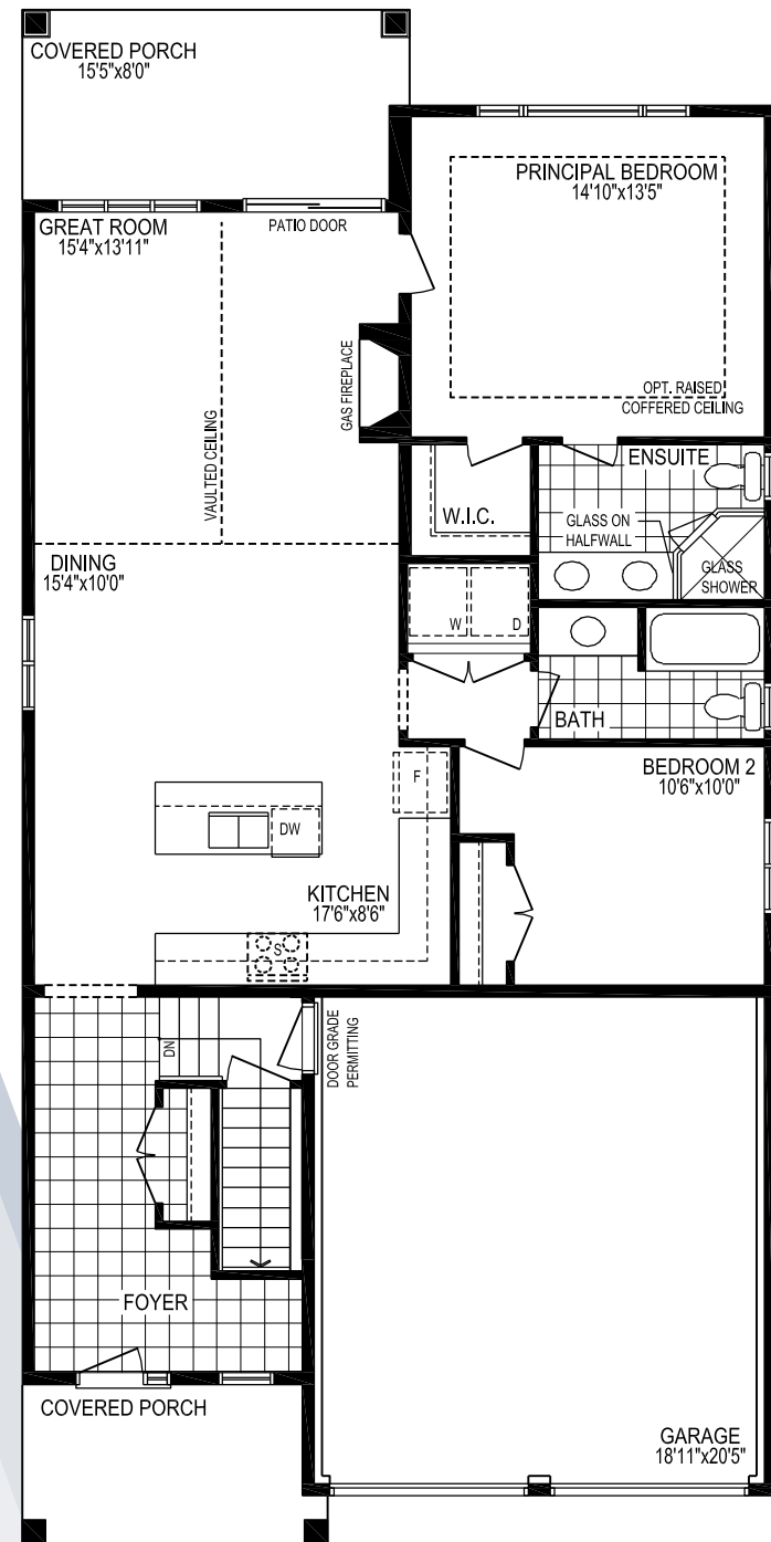
GROUND FLOOR PLAN, EL. 'A' (*'B' SIMILAR)
