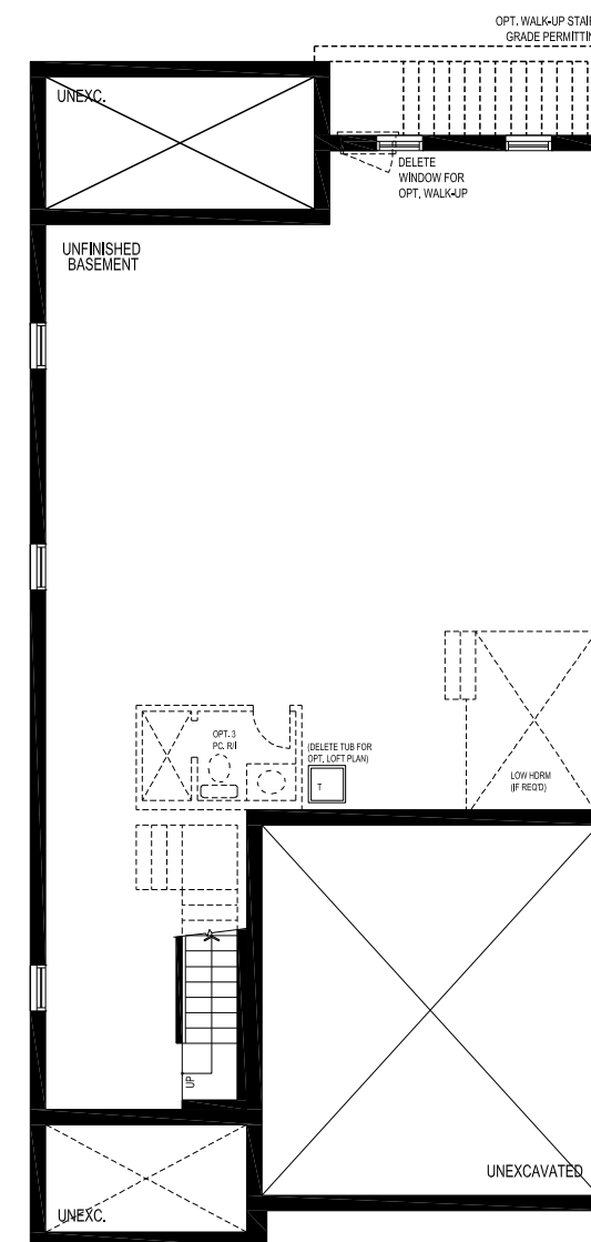
BASEMENT PLAN, EL. 'A' & 'B'
