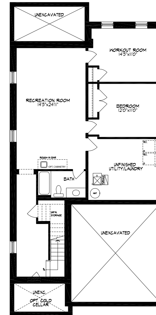
OPT. FINISHED BASEMENT PLAN, EL. 'A' & 'B'
