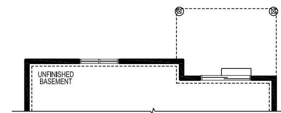
PART. BASEMENT PLAN EL. 'A' 'B' & 'C' - WALK-OUT CONDITION
