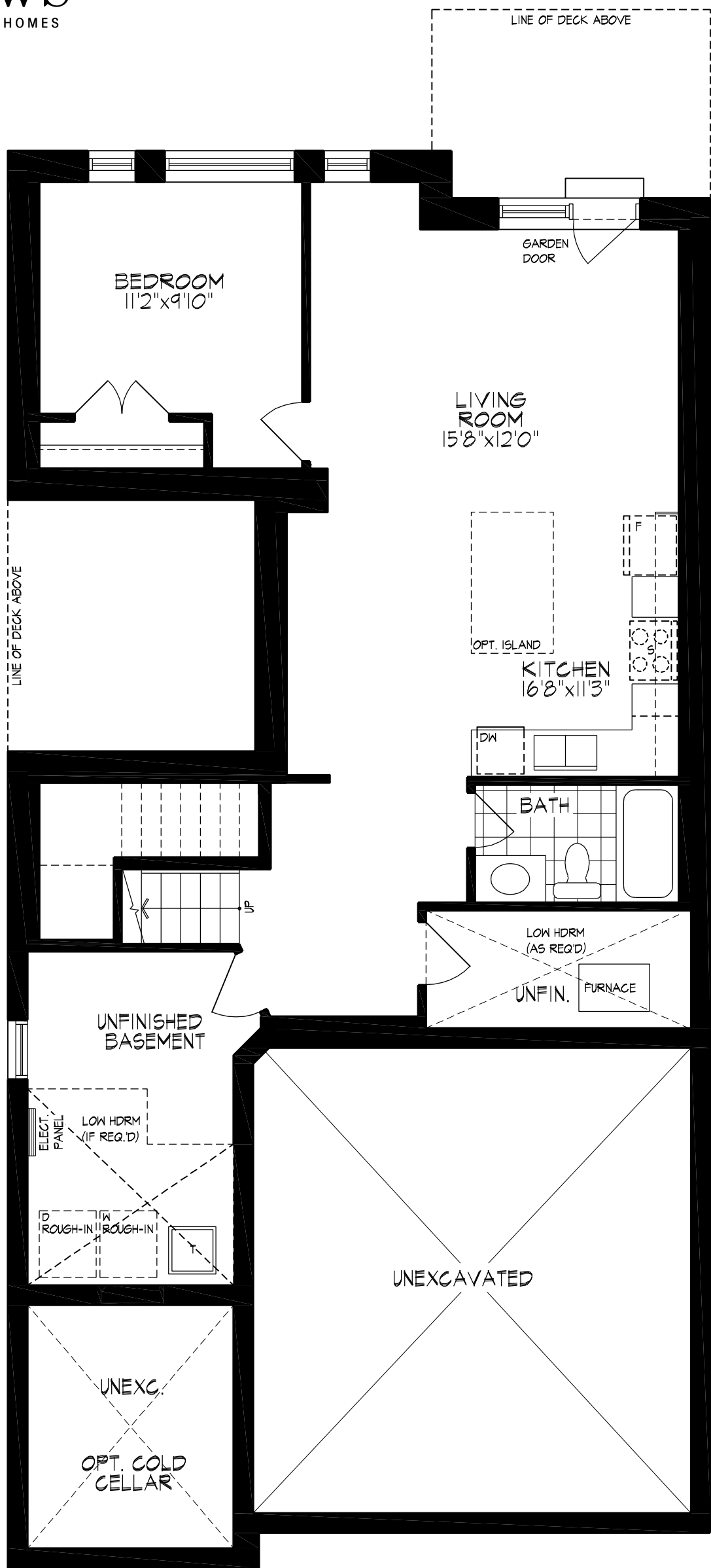
FINISHED BASEMENT PLAN
