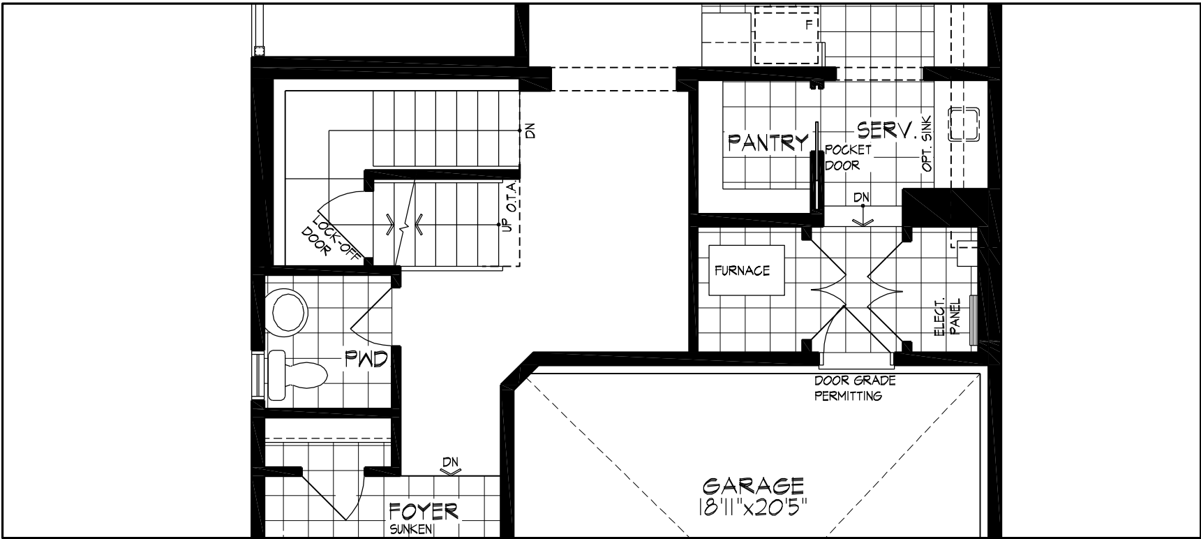
GROUND FLOOR PLAN FOR FINISHED BASEMENT
