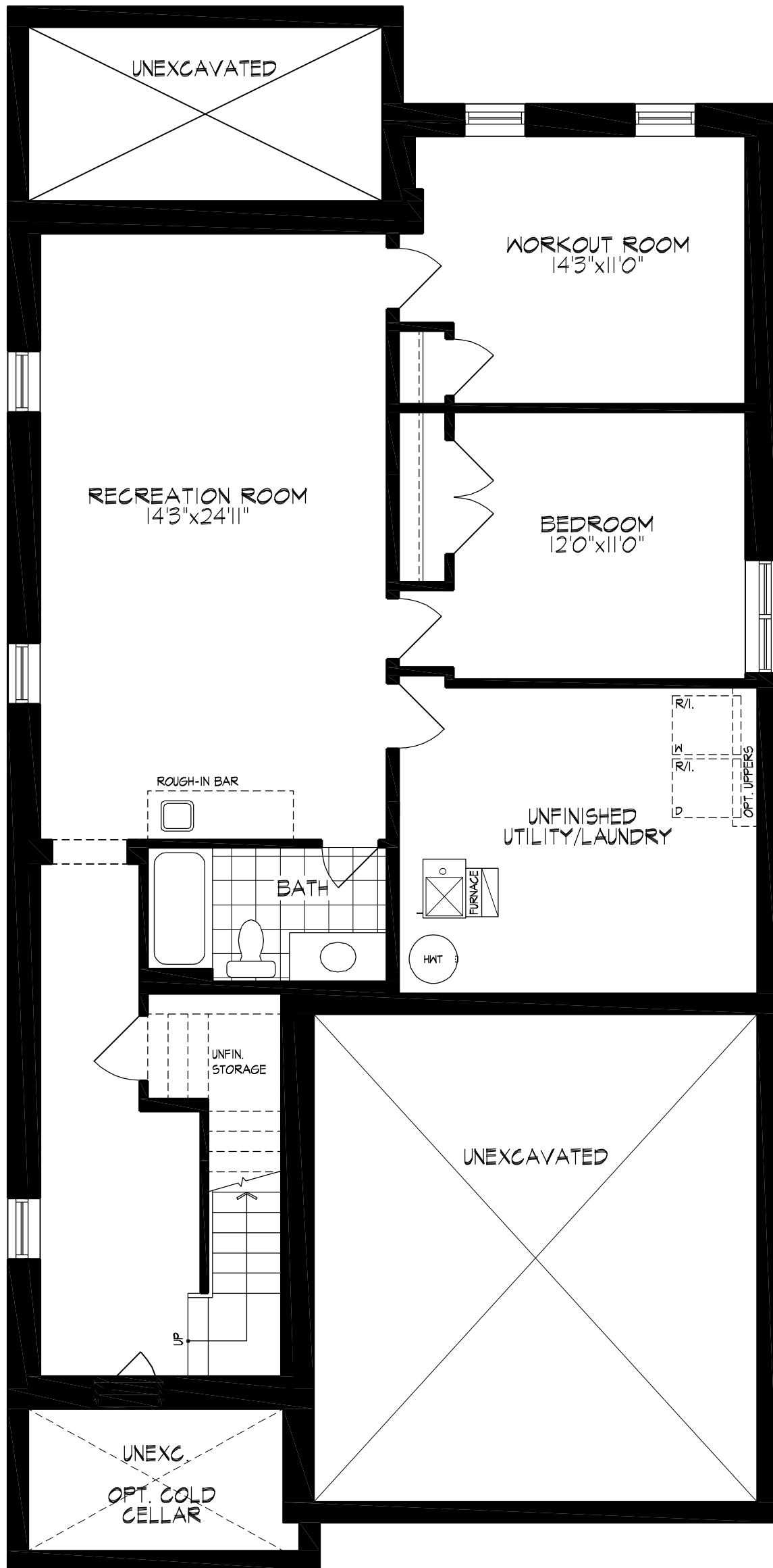
FINISHED BASEMENT PLAN
