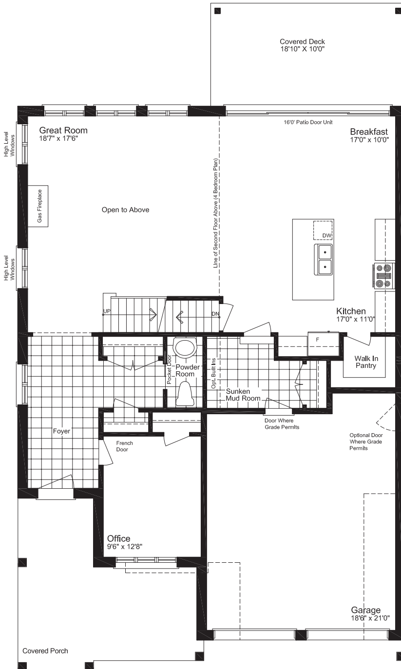
GROUND FLOOR PLAN 'A' & 'B'
