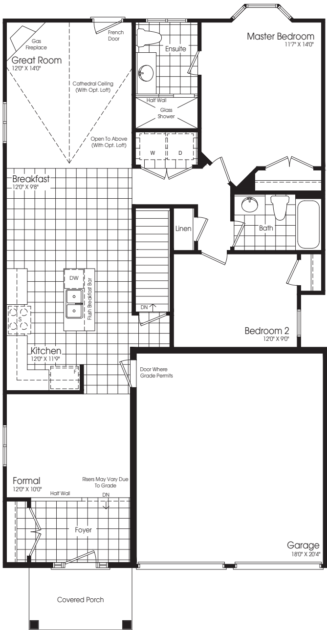
GROUND FLOOR PLAN 'A'
