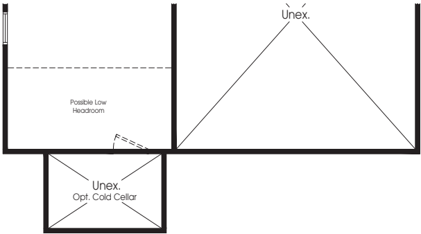
PARTIAL BASEMENT PLAN 'A'
