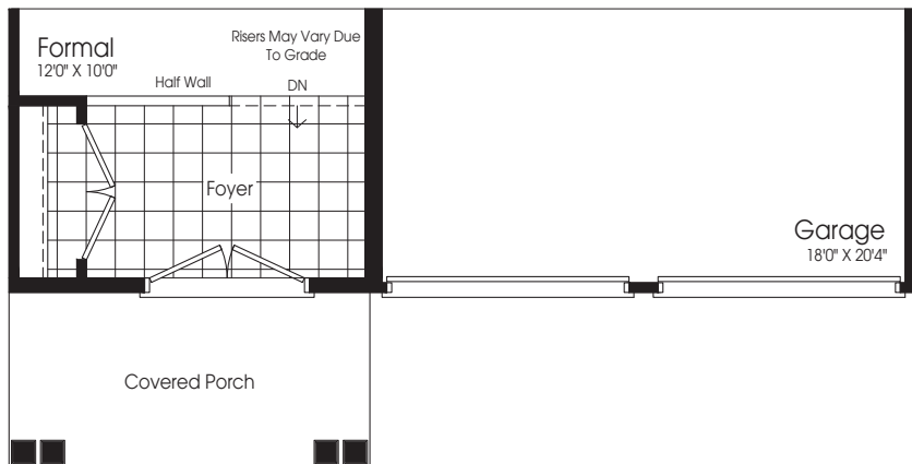
PARTIAL GROUND FLOOR PLAN 'B'
