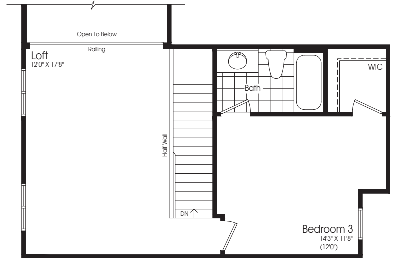
OPT. LOFT FLOOR PLAN 'A' & 'B'
