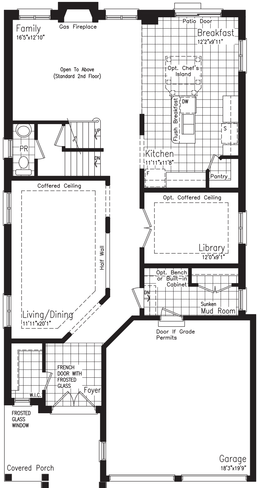
GROUND FLOOR PLAN 'A' & 'B'
