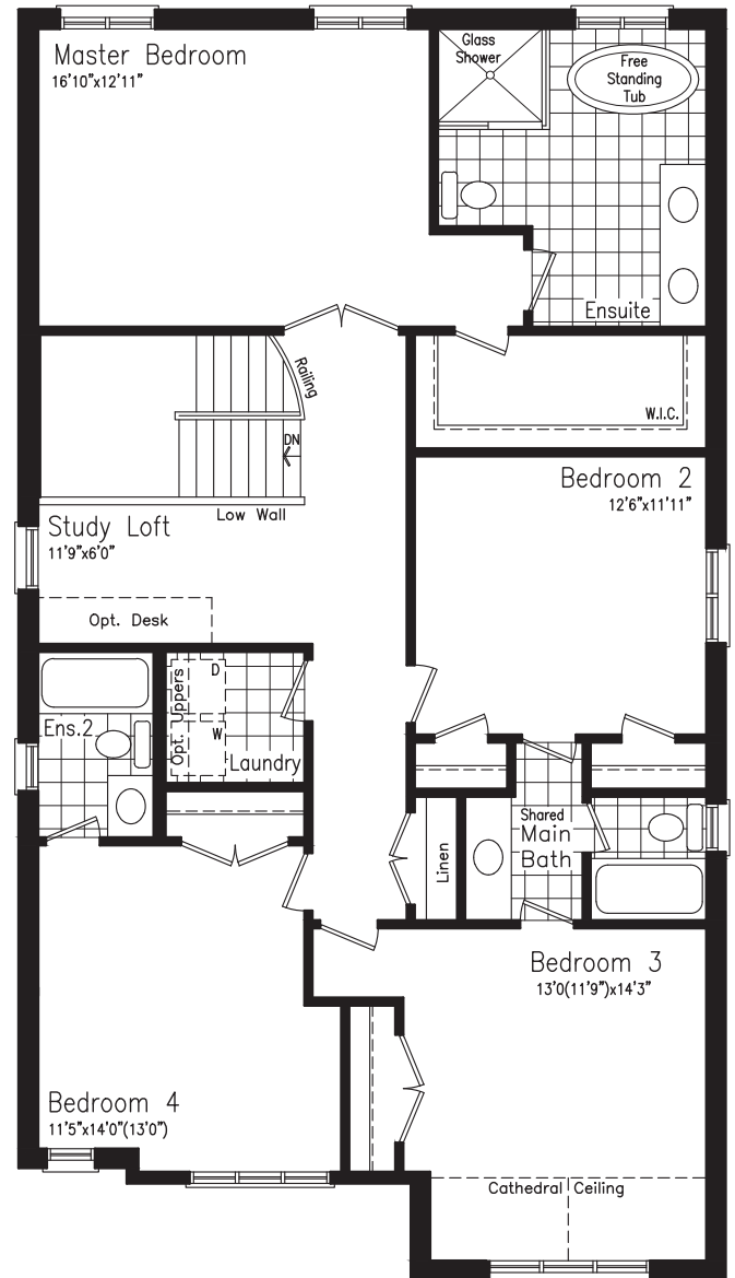
OPTIONAL 2ND FLOOR PLAN 'A' & 'B'
