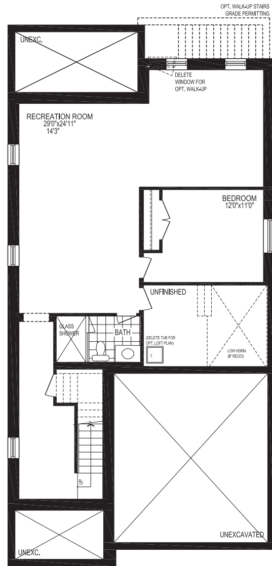
OPT. FINISHED BASEMENT PLAN, EL. 'A' & 'B'
