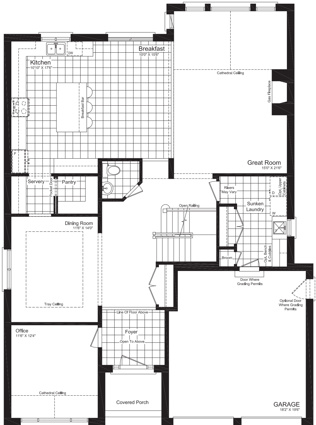
GROUND FLOOR PLAN 'C'
