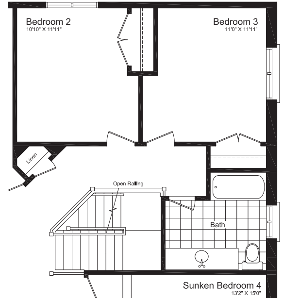
PARTIAL OPTIONAL SECOND FLOOR PLAN
